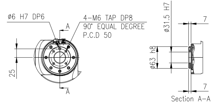
Detail A (TOOL FLANGE) (Scale 1/5)
