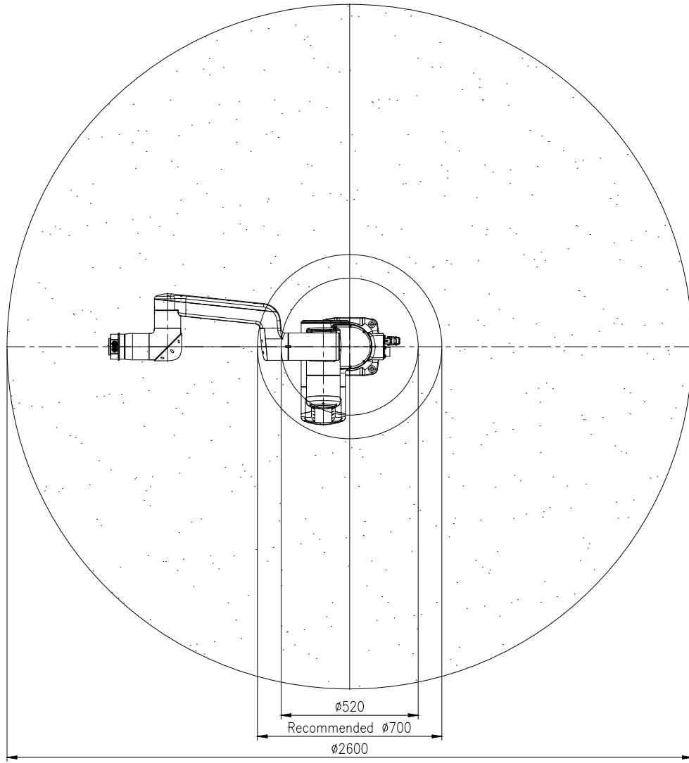
HCR-12 Working area, top view
