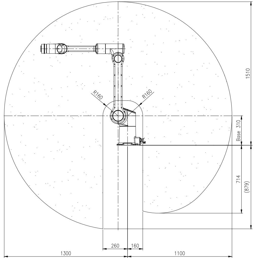
HCR-12 Working area, side view
